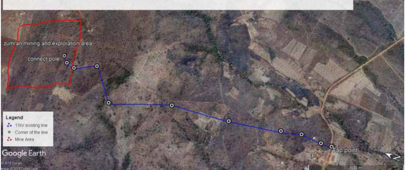
THE CONSTRUCTED 11KV OVERHEAD LINE FROM CHIKWAMA PRIMARY SCHOOL TO ZUMRAN MINE
